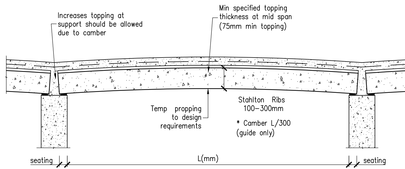
CAMBER (HOG) ALLOWANCE
