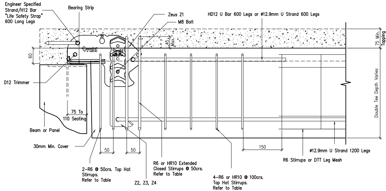
Double Tee End Seating with Zues bracket
