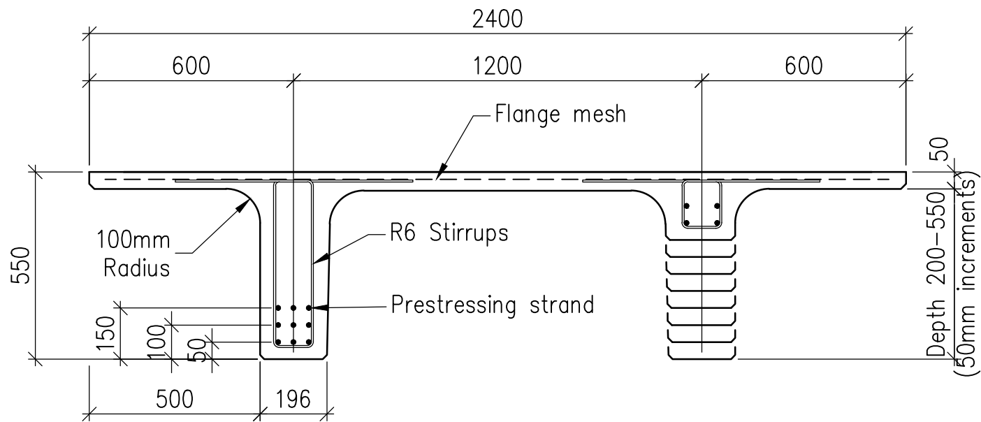
Stahlton Double Tee Typical Section Scale 1:15
