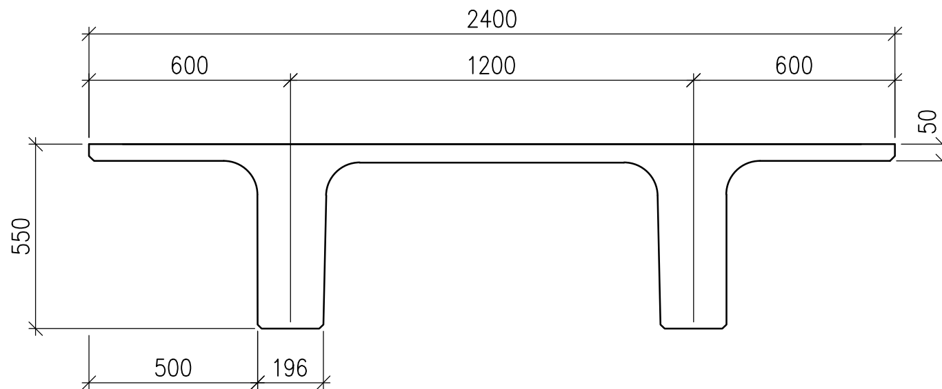
550 Double Tee Typical Section Scale 1:15
