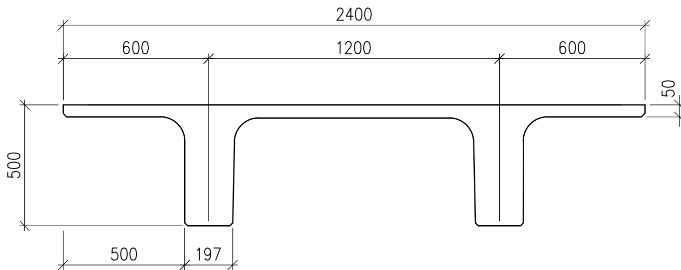
500 Double Tee Typical Section Scale 1:15
