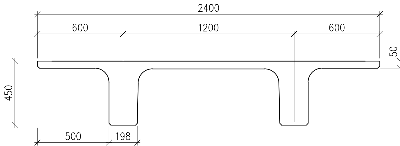
450 Double Tee Typical Section
