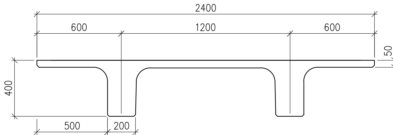
400 Double Tee Typical Section
