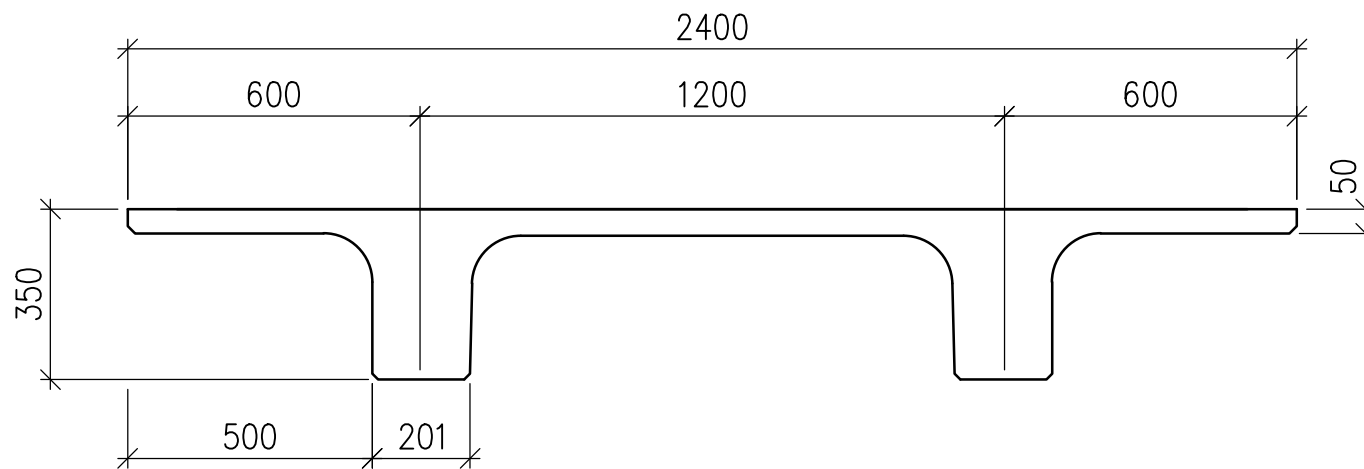
350 Double Tee Typical Section
