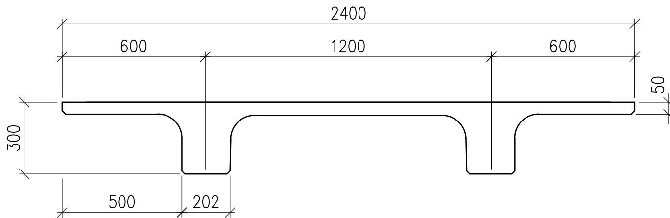
300 Double Tee Typical Section Scale 1:15
