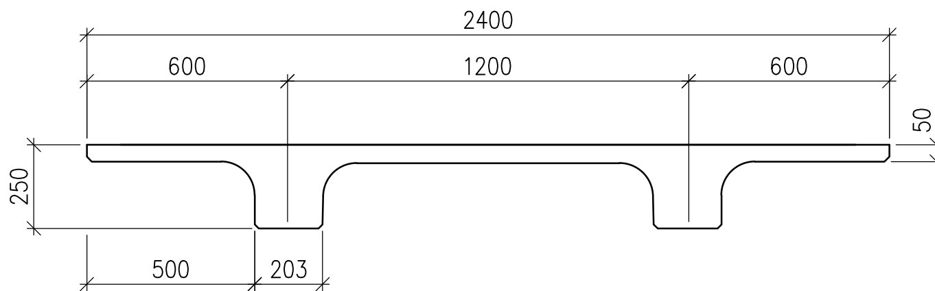
250 Double Tee Typical Section
