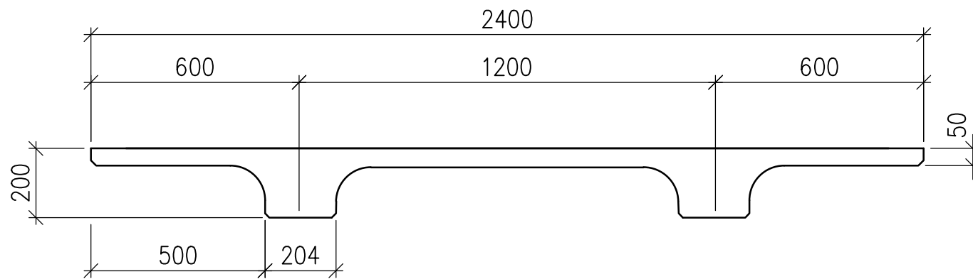
200 Double Tee Typical Section Scale 1:15
