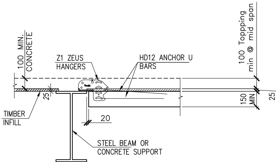
RIB ZEUS SEATING DETAIL Scale 1 : 20
