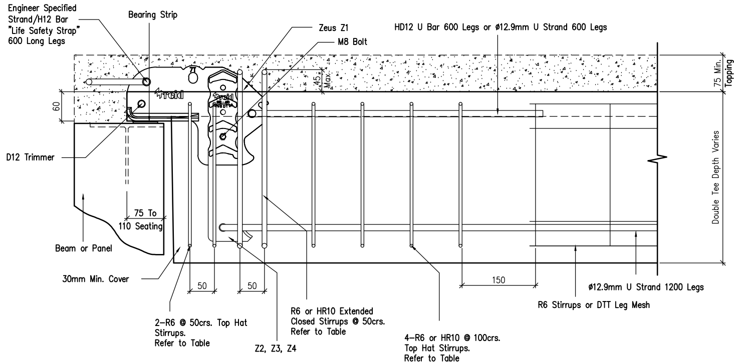
Double Tee End Seating with Zues bracket
