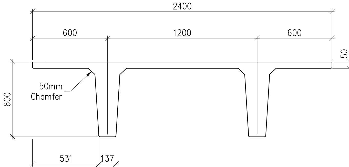
600 Double Tee Typical Section – CHC Option only
