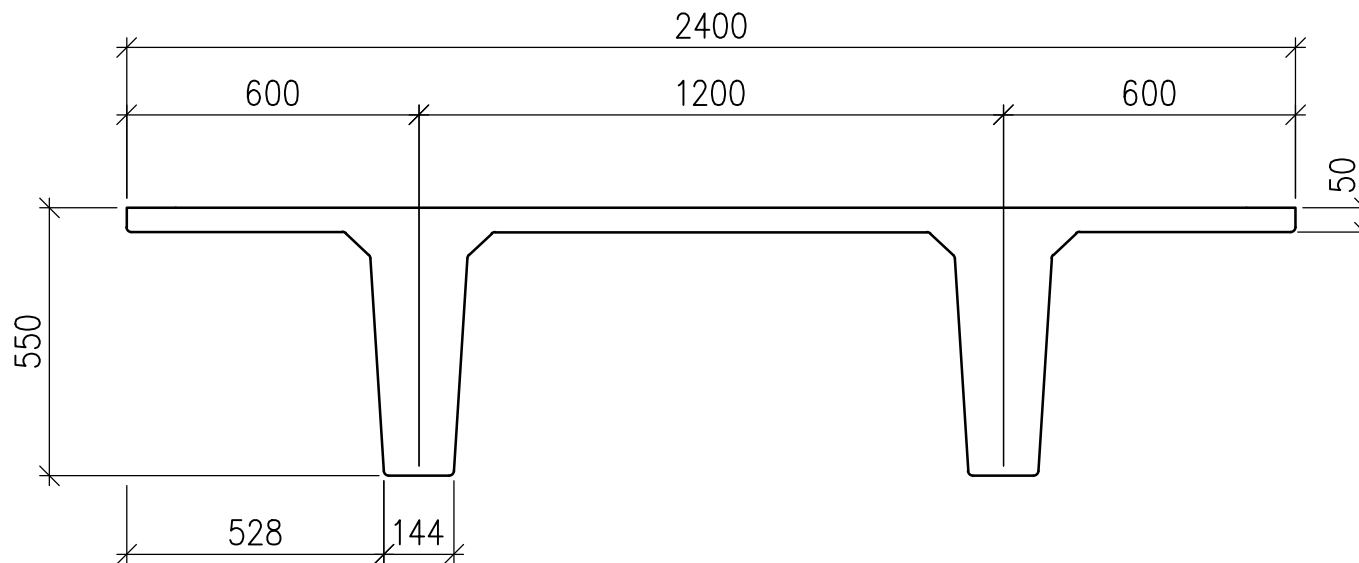
550 Double Tee Typical Section – CHC Option only Scale 1:15
