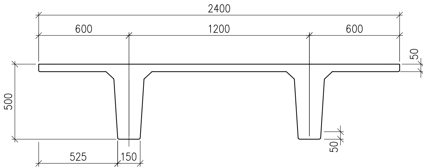
500 Double Tee Typical Section – CHC Option only
