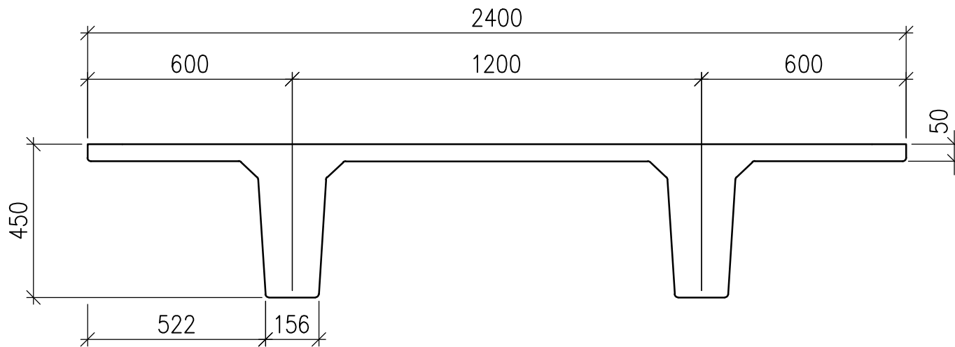
450 Double Tee Typical Section – CHC Option only
