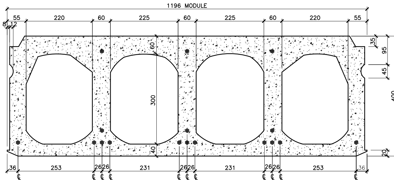
400 ELESTATIC SLAB
