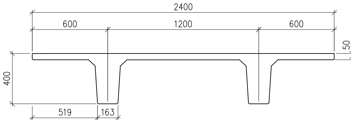
400 Double Tee Typical Section – CHC Option only
