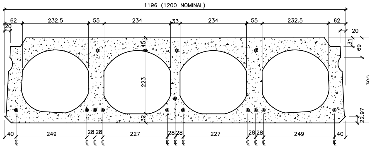
300 ELEMATIC SLAB
