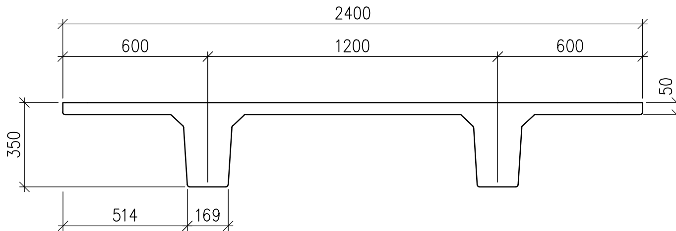
350 Double Tee Typical Section – CHC Option only
