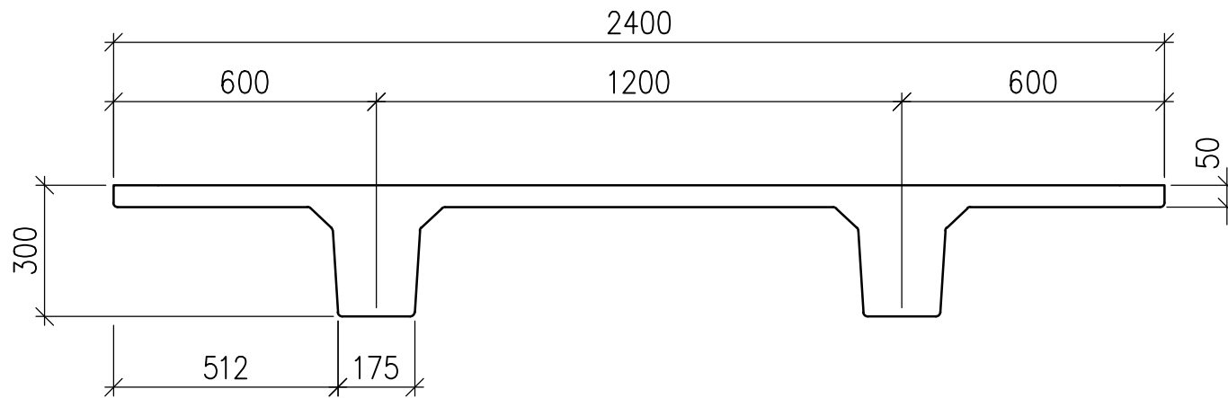
300 Double Tee Typical Section – CHC Option only
