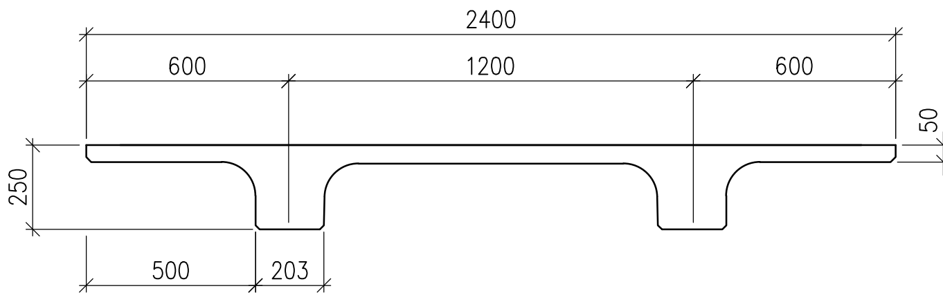
250 Double Tee Typical Section Scale 1:15
