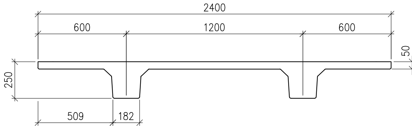
250 Double Tee Typical Section – CHC Option only Scale 1:15
