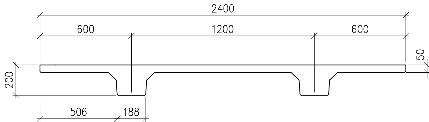
200 Double Tee Typical Section – CHC Option only Scale 1:15
